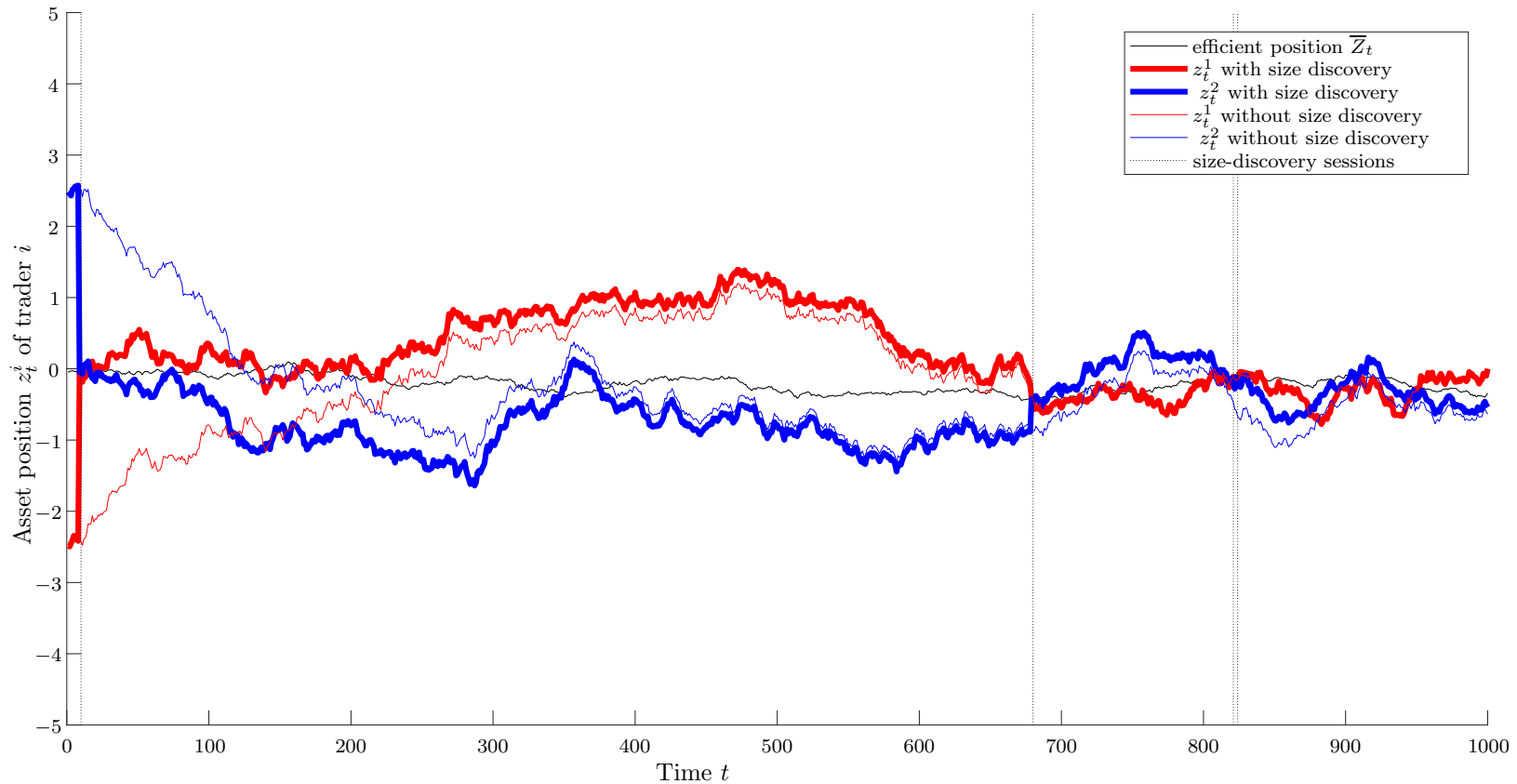
Figure 2: Inventory sample paths with and without size-discovery. This figure plots the inventory sample paths of two of the n = 10 traders, with and without size-discovery mechanisms, based on the equilibria characterized by Propositions 4 and 3, respectively. For each trader, the inventory shock process is an independent Brownian motion with standard-deviation parameter \sigma_i = 0.05 . The aggregate inventory is an independent Brownian motion with standard-deviation parameter \sigma_Z = 0.15 . The other parameters are mean asset payoff v = 0.5 , mean rate of arrival of asset payoff r = 0.1 , inventory cost coefficient \gamma = 0.1 , initial aggregate market inventory Z_0 = -0.5 , an initial asset position of trader 1 of z_0^1 = -2.5 , an initial asset position of trader 2 of z_0^2 = 2.5 , and a mean frequency \lambda = 0.1167 = 0.99\bar{\lambda} of size-discovery sessions. The graphs of the asset positions are shown in heavy line weights for the market with optimal size-discovery mechanisms, and in light line weights for the market with no size-discovery sessions.
