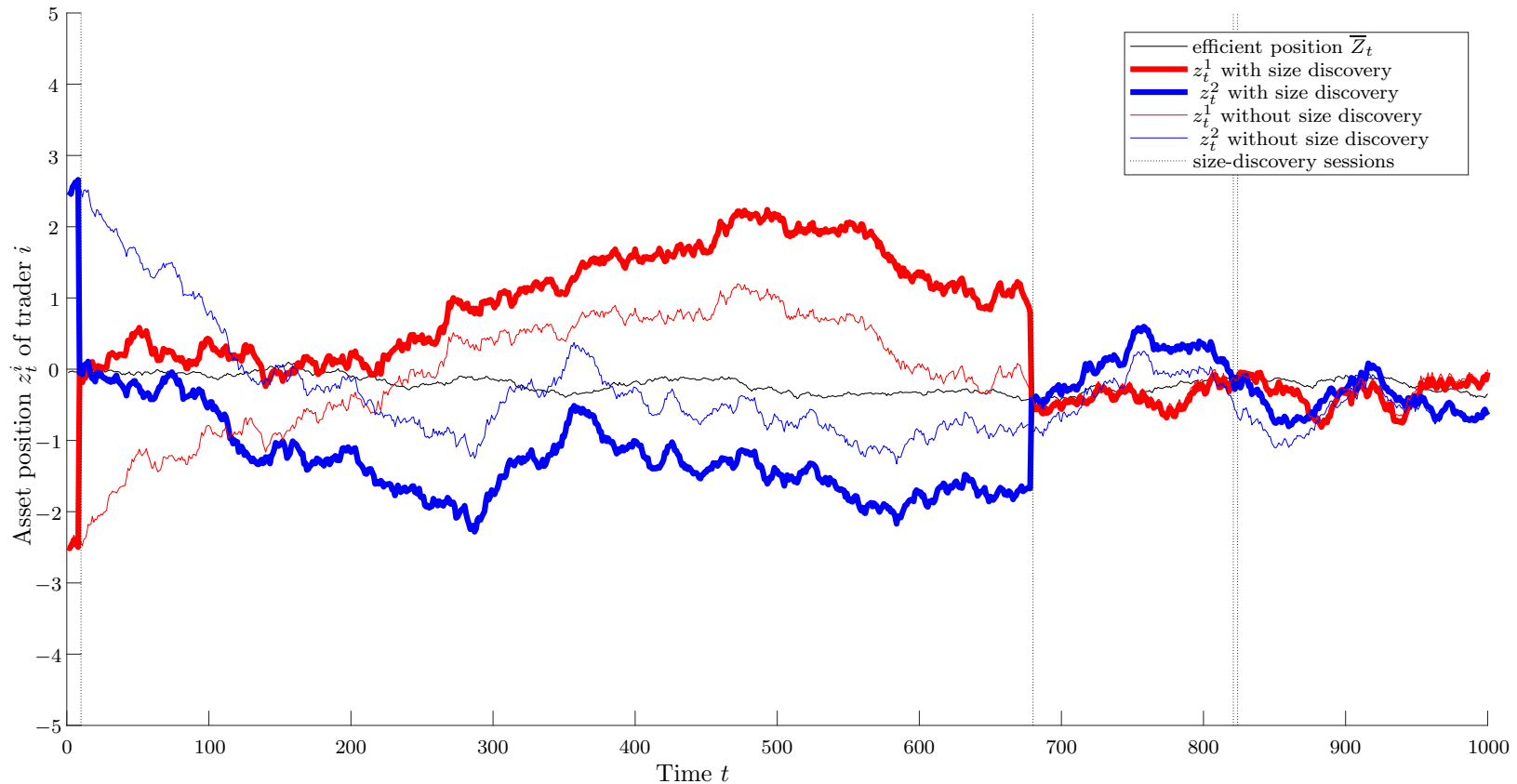
Figure 3: Inventory sample paths with and without price-based size discovery. This figure plots the inventory sample paths of two of the n = 10 traders, with and without size-discovery mechanisms, based on the equilibria characterized by Propositions 5 and 3, respectively. For each trader, the inventory shock process is an independent Brownian motion with standard-deviation parameter \sigma_i = 0.05 . The aggregate inventory is an independent Brownian motion with standard-deviation parameter \sigma_Z = 0.15 . The other parameters are mean asset payoff v = 0.5 , mean rate of arrival of asset payoff r = 0.1 , inventory cost coefficient \gamma = 0.1 , initial aggregate market inventory Z_0 = -0.5 , an initial asset position of trader 1 of z_0^1 = -2.5 , an initial asset position of trader 2 of z_0^2 = 2.5 , and a mean frequency \lambda = 0.1167 = 0.99\bar{\lambda} of size-discovery sessions. The graphs of the asset positions are shown in heavy line weights for the market with optimal size-discovery mechanisms, and in light line weights for the market with no size-discovery sessions.
